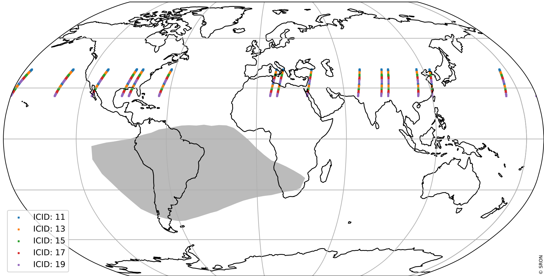
ground-tracks of Sentinel-5P
